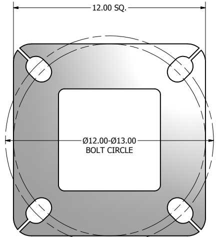
12.00 X 12.00 X 1.00 THK. BASE PLATE
